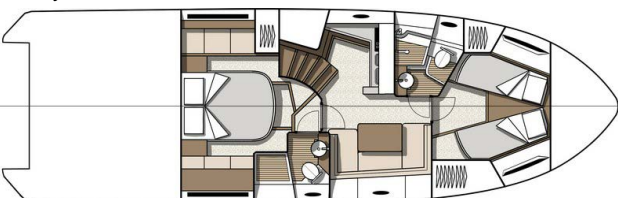
2 cabin layout
