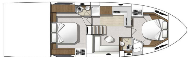
2 cabins layout
